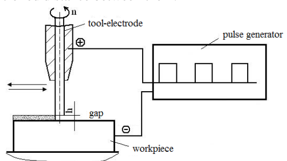
Fig. 5. The workscheme of surface hardening by pulsed electric discharge machining (Topala, 2008)
